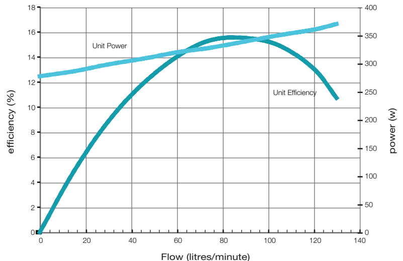
Efficiency Chart
