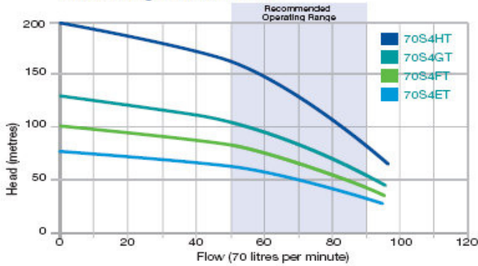
70S4 Range Performance
