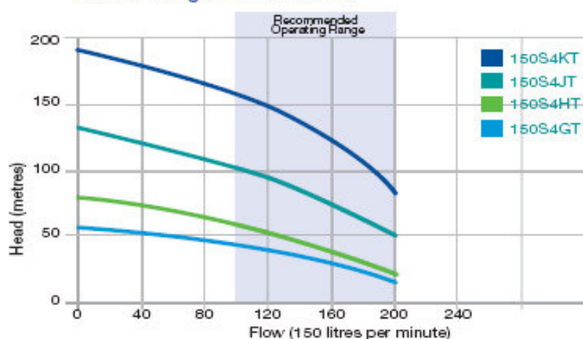
150S4 Range Performance
