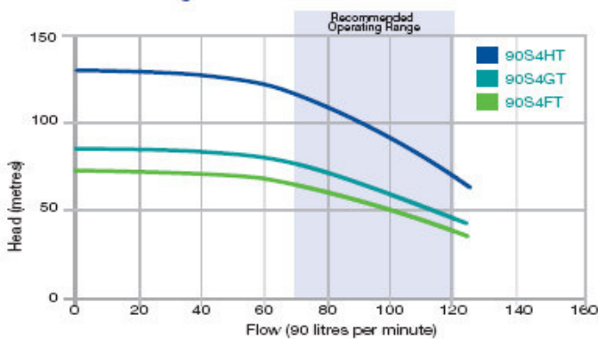
90S4 Range Performance
