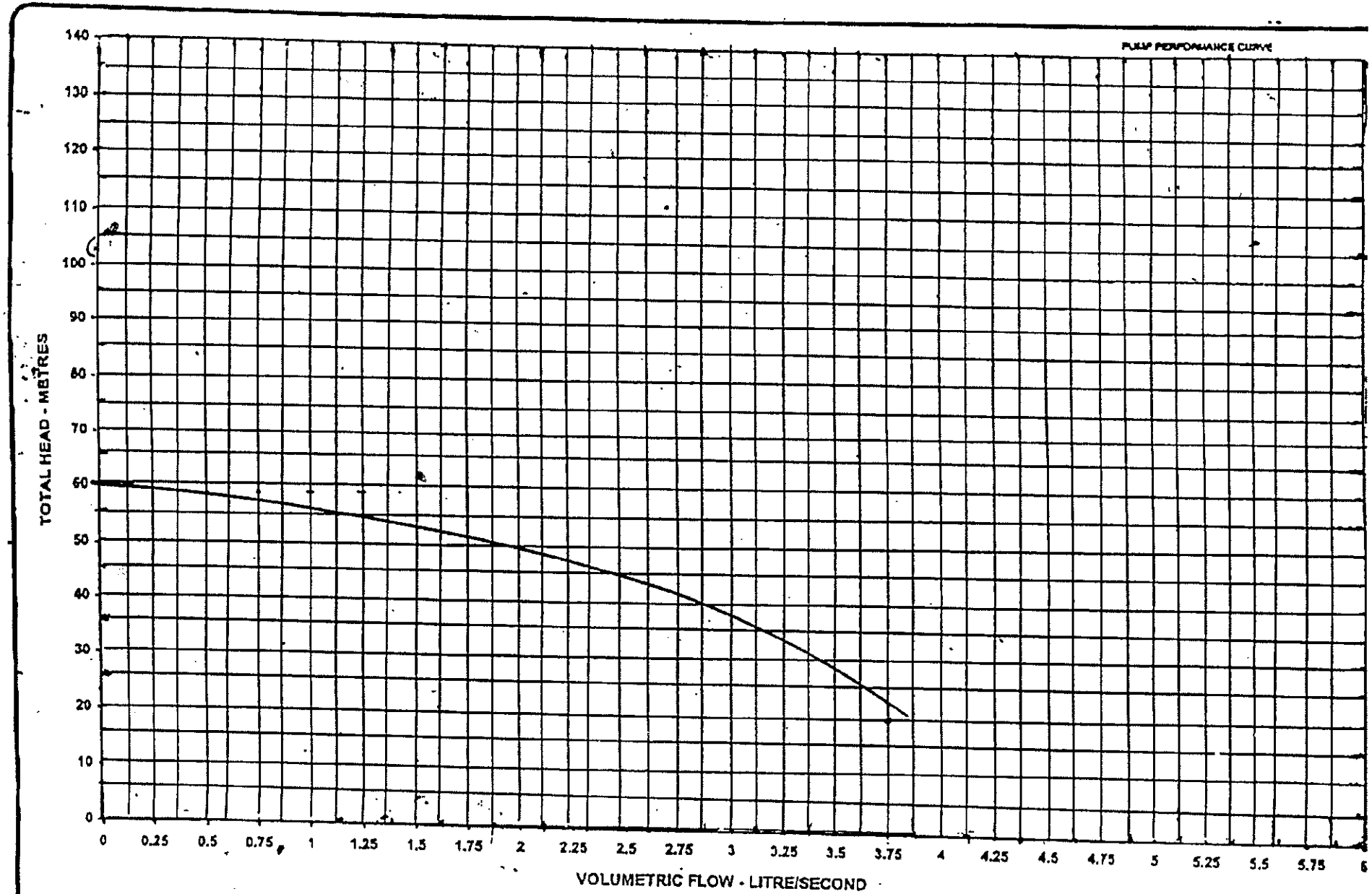
VILLIERS TWIN IMPELLER FIRE-FIGHTER PUMP
